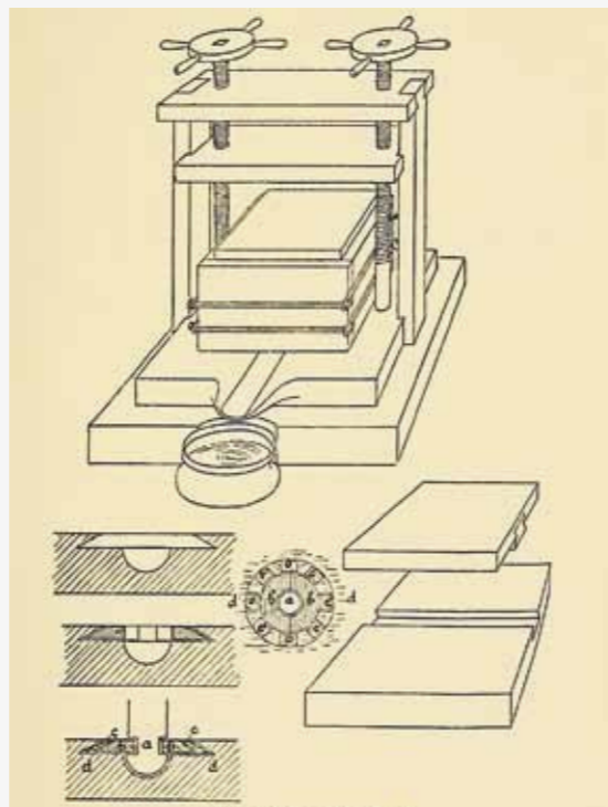
FIG. 12.—Small screw press.
